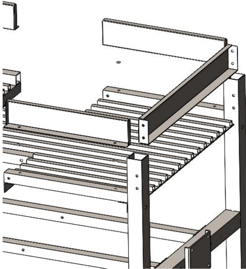
Detail view 2
