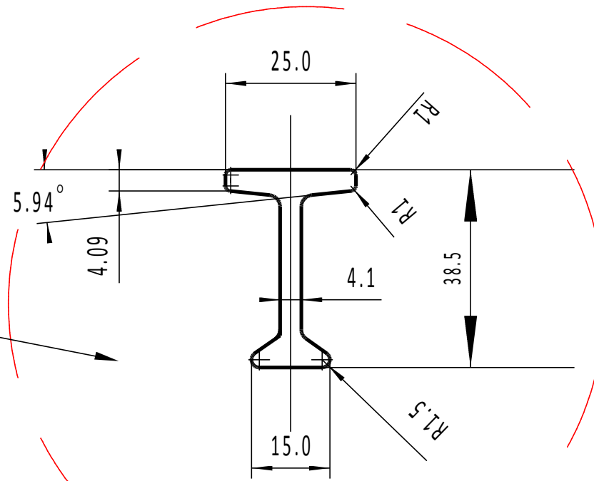
I-bar's Details
